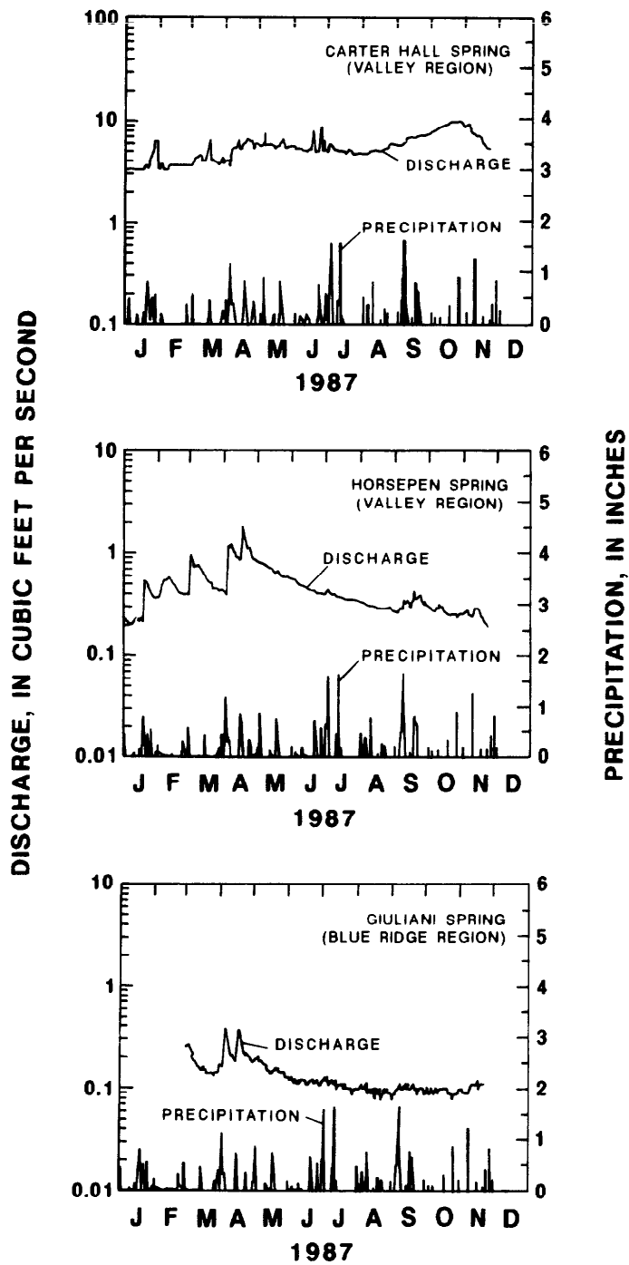
Figure 12--Discharge hydrographs for three springs in Clarke County, Virginia, and precipitation at Blandy Farm, 1987.
