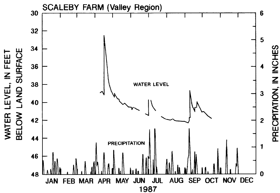
Figure 10.--Hydrograph for a well at Scaleby Farm in Clarke County, Virginia, and precipitation at Blandy Farm, 1987.
